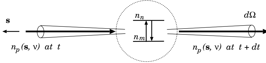
Figure 19: Time variation of the number density of photons.
