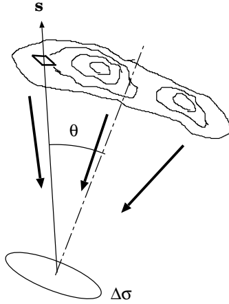
Figure 10: Definition of spectral flux density \mathcal{S}_\nu .
