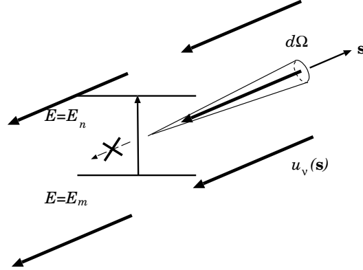
Figure 16: Absorption of radiation.
