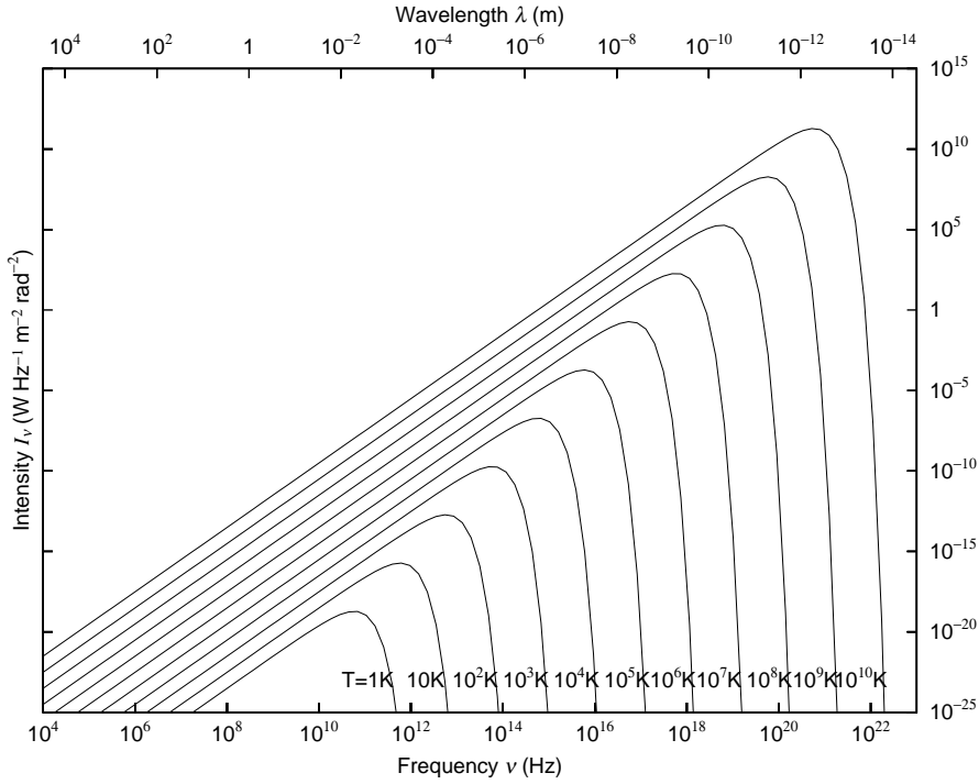
Figure 20: Planck spectrum of the intensity of the black body radiation. Each curve corresponds to a certain absolute thermodynamic temperature value.
