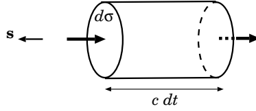
Figure 11: Radiation energy per unit solid angle in a tube.
