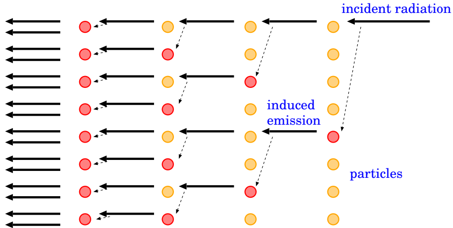
Figure 24: A schematic view of maser amplification. Induced emission causes new induced emission, initiating an “avalanche” of maser emission photons all traveling in a common direction parallel to the incident photon.
