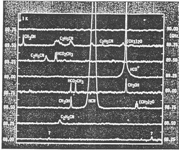
Figure 3: Thermal molecular lines observed in the Orion-KL star-forming region (Kaifu et al., 1985).
