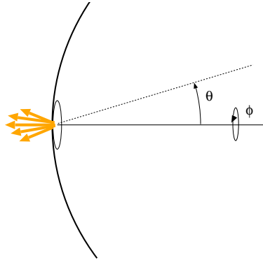
Figure 22: Thermal radiation from a surface of a black body.
