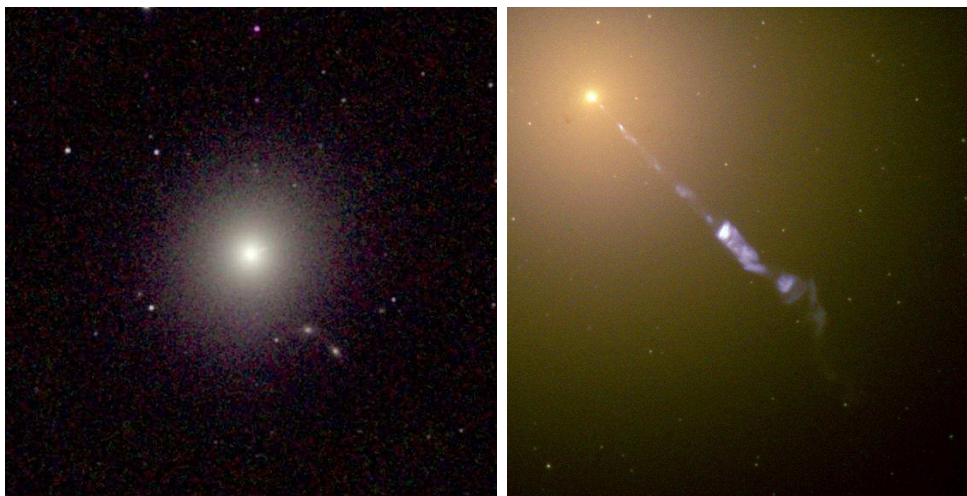
Figure 27: Many galaxies show activity in their nuclei, involving violent ejections of high-energy electrons and resultant synchrotron radiation. A nearby galaxy M87, also known as Virgo A or 3C 274 in radio astronomy, is an example. Left: Infrared image of M87 by 2 Micron All Sky Survey (2MASS). Right: Close-up view of a collimated jet by Hubble Space Telescope (HST). (Figure courtesy of NASA/IPAC Extragalactic Database (NED) operated by the Jet Propulsion Laboratory, California Institute of Technology, under contract with the National Aeronautics and Space Administration).
