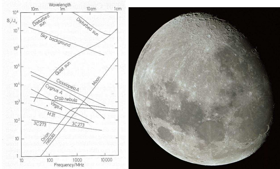
Figure 21: Spectra of continuum radio sources (Kraus, 1986; Left), and an optical image of the Moon (Right). Do we see such a halfmoon image in radio waves?
