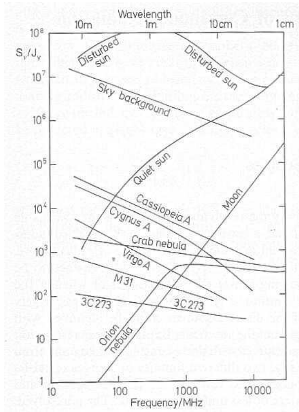
Figure 2: Spectra of galactic and extragalactic continuum radio sources (from Kraus, 1986).
