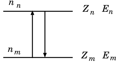
Figure 18: Number densities of particles in the two energy states.
