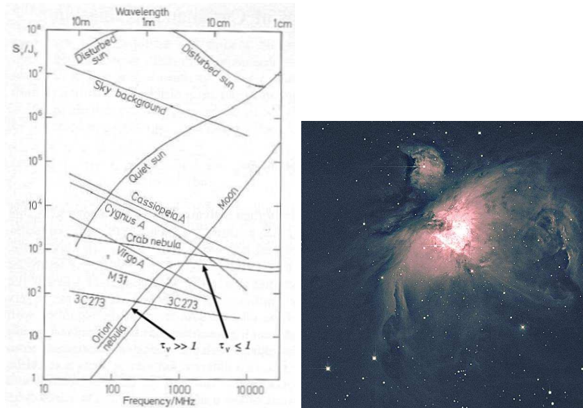
Figure 26: Interpretation of the spectrum of the Orion Nebula. Left panel is from Kraus (1986).
