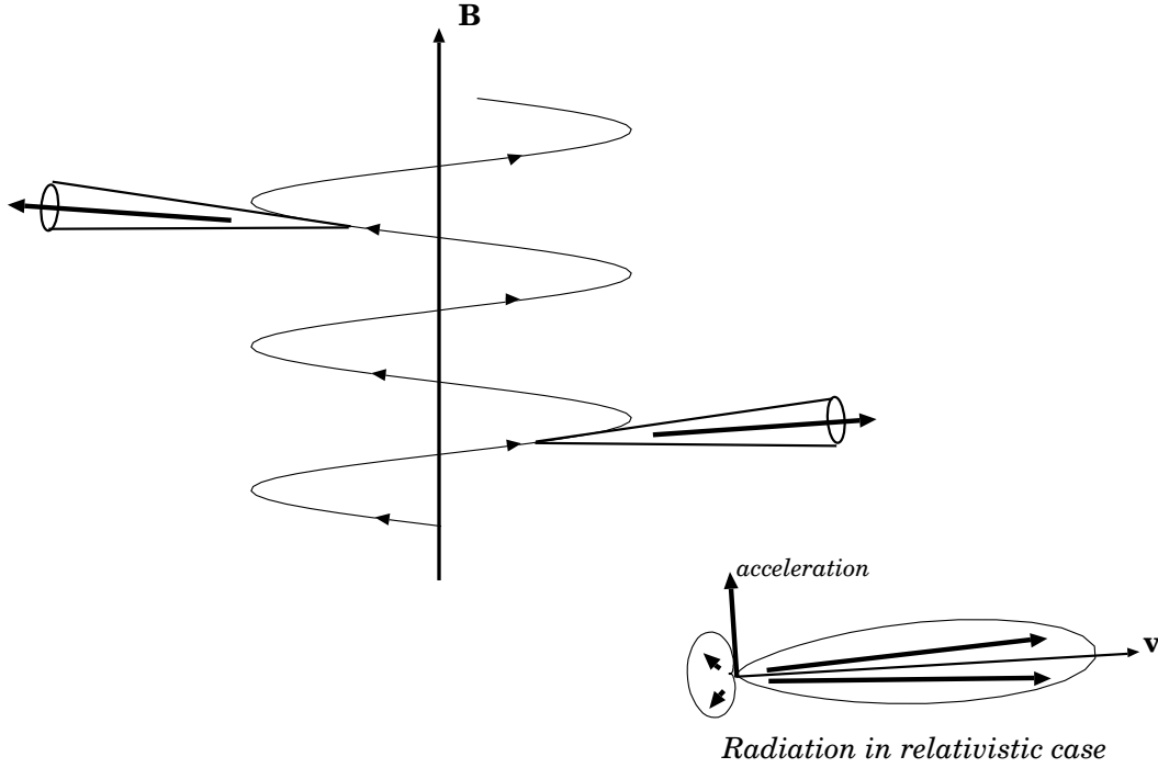
Figure 29: Synchrotron radiation from a relativistic electron.
