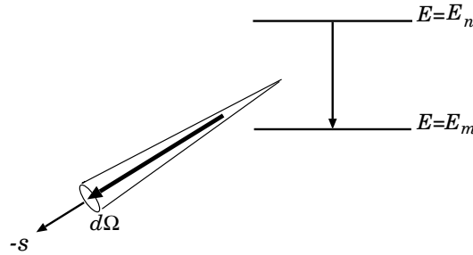
Figure 15: Spontaneous emission of radiation.
