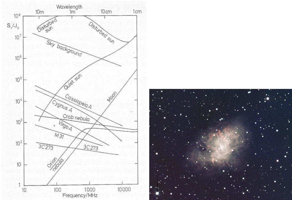
Figure 30: Spectra of continuum radio sources, including non-thermal sources with positive spectral indices (Kraus, 1986; Left), and the Crab Nebula supernova remnant, a typical synchrotron radiation source.
