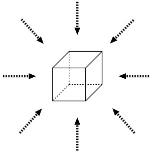
Figure 12: Spectral energy density: energy of radiation coming from all directions, contained in a unit volume.
