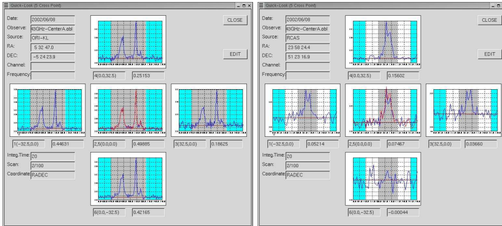
Figure 5: SiO maser lines in Orion-KL (Left), and R Cas (Right) observed in pointing tests for a VERA antenna (courtesy of VERA group, Japan, 2002).
