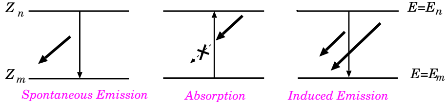
Figure 14: The three possible transitions between two energy states.
