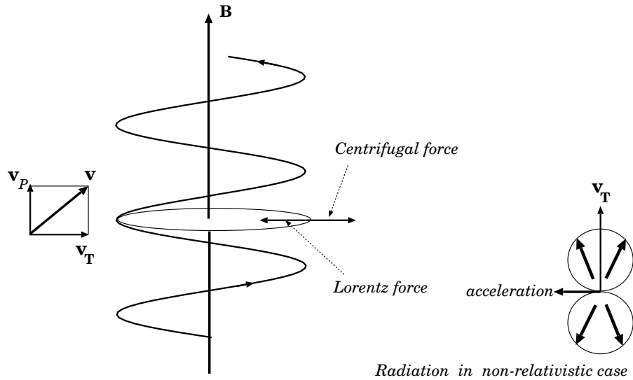
Figure 28: “Cyclotron” or “Gyro-synchrotron” radiation
