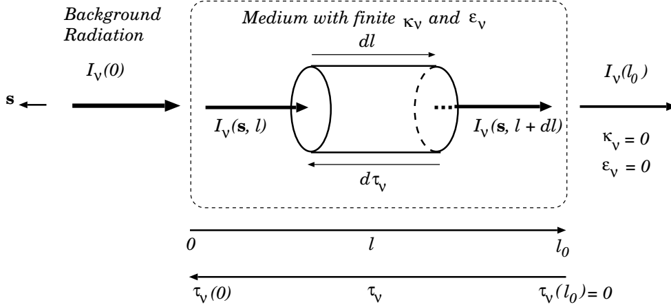
Figure 25: Radiative transfer in LTE and optical depth.
