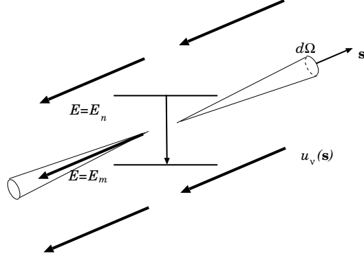
Figure 17: Induced (or stimulated) emission of radiation.
