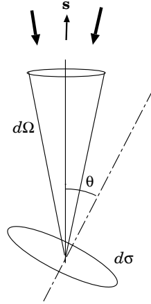
Figure 8: Power dW of radiation with Specific/Monochromatic Intensity I_\nu(\mathbf{s}) (or Brightness B_\nu(\mathbf{s}) ) coming through a solid angle d\Omega , a cross-section d\sigma , and a frequency bandwidth d\nu is given by dW = I_\nu(\mathbf{s}) \cos \theta d\Omega d\sigma d\nu .
