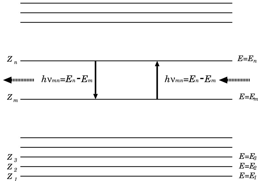
Figure 13: Energy levels and transitions with emission (left-hand arrow) or absorption (right-hand arrow) of radiation.
