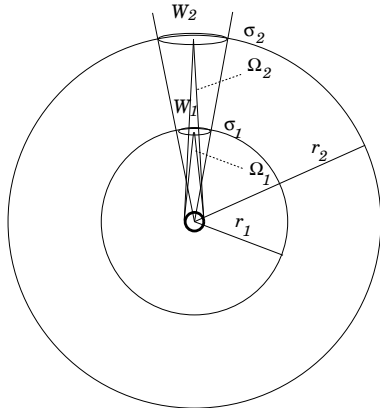
Figure 9: Constancy of the monochromatic intensity I_\nu along the ray path.
