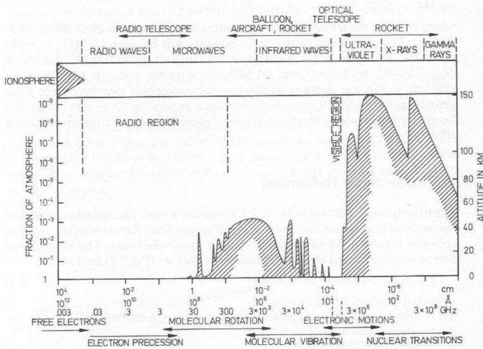
Figure 1: ‘Windows’ for ground-based astronomy (from Rohlfs & Wilson, 2001).
