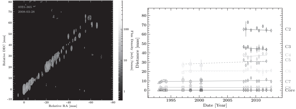
Fig. 1. Left panel : TANAMI full-resolution 8.4 GHz images of PKS 0521–36. The contours start at 3 times the rms level. The beam size is indicated in grey in the lower left corner. Right panel : Results of the preliminary kinematic analysis for PKS 0521–36, including TANAMI data and previous VLBI data from [22]. The plot shows the distance of jet component relative to the core as a function of time.
